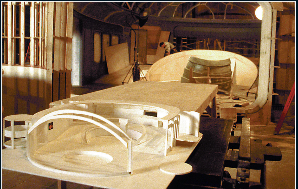
► The study model for the bridge in front of the real thing, while it was under construction.
